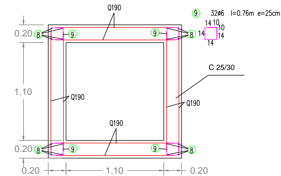
armaturne mreže-B500A(MAG500/560)
